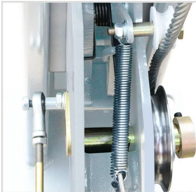
Rapid-Descent Protection mechanism
