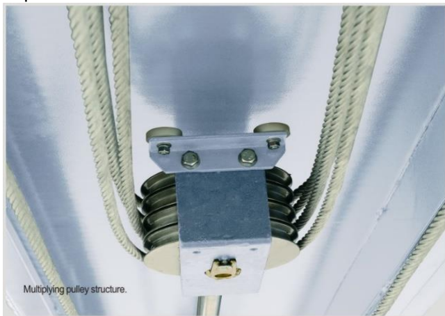
Multiplying pulley
